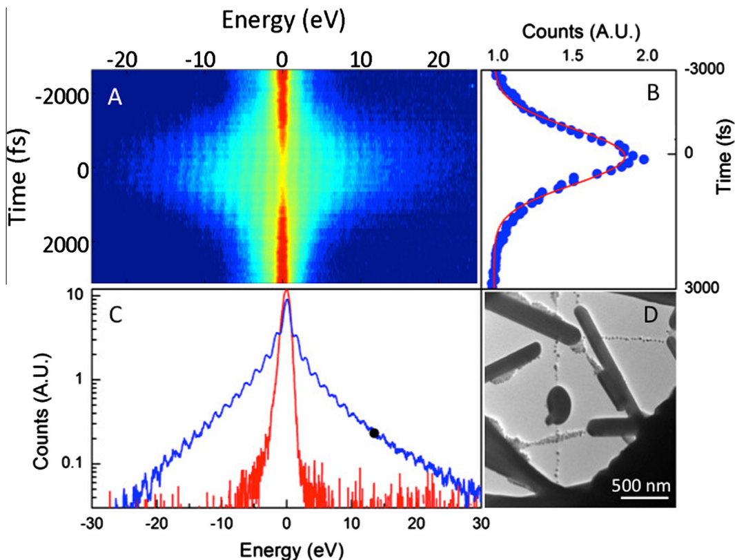
Fig. 3. (A) Time/energy landscape of the PINEM effect on silver nanotubes. (B) temporal profile of one of the PINEM sidebands. (C) Energy profile of the PINEM spectrum. (D) Image of the silver nanowires acquired using photoemitted electrons.
