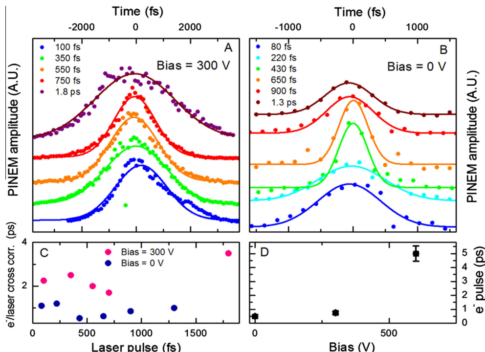
Fig. 4. (A) Temporal profile of the amplitude of a PINEM sideband as a function of the laser pulses duration at a bias voltage of 300 V. The peak intensity of the pump is kept constant. (B) Temporal profile of a PINEM sideband as a function of the laser pulses duration at a bias voltage of 0 V. (C) FWHM of the PINEM temporal profile as a function of the laser pulse duration for two bias voltages. (D) The shortest electron pulse duration obtained at the different bias voltages is plotted against the bias.
