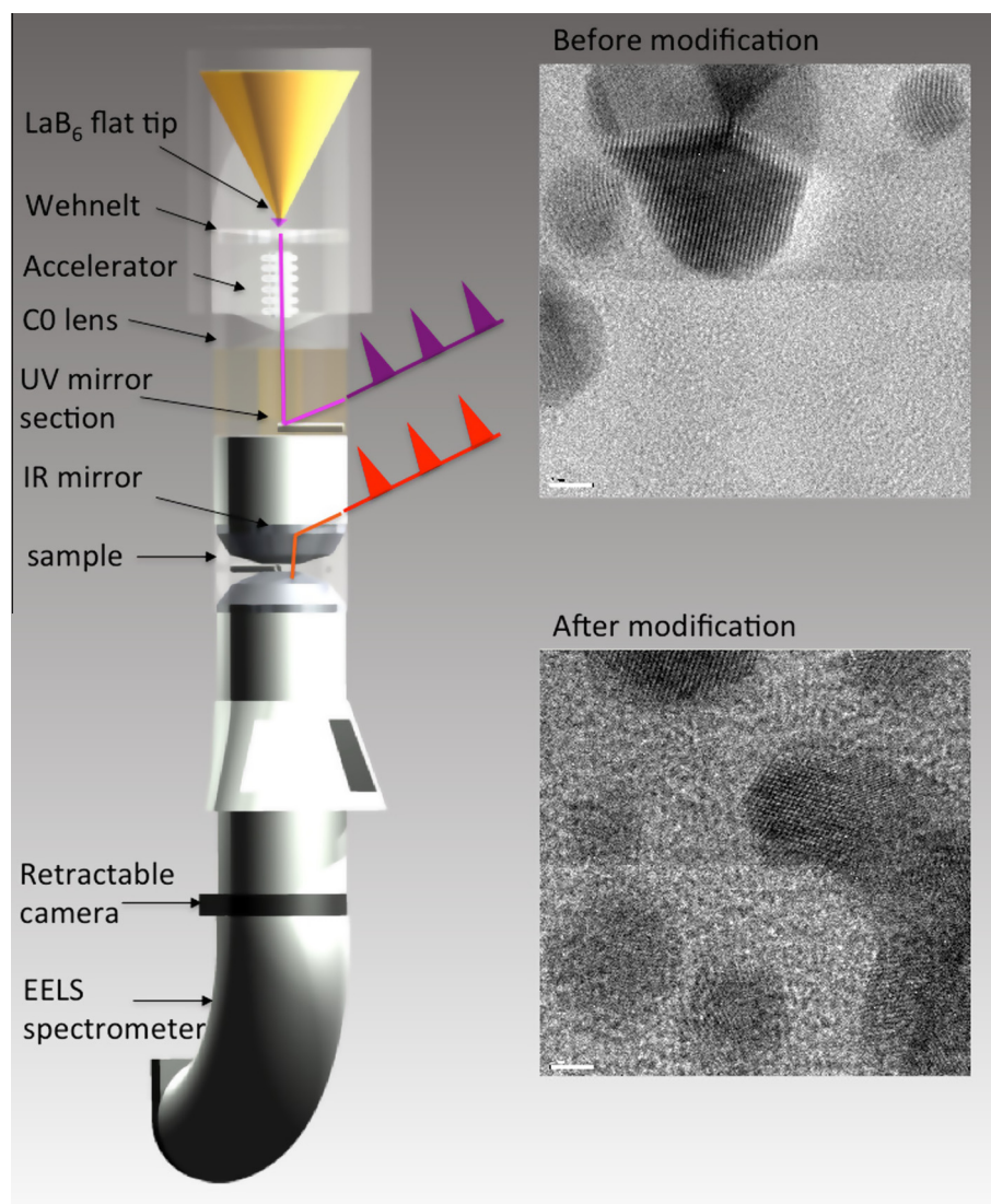
Fig. 1. Modified TEM: the critical sections where conventional parts have been modified are transparent. In the right panel a static atomic resolution image taken on a gold nano-particle TEM resolution standard is shown before and after the modification of the instrument.
