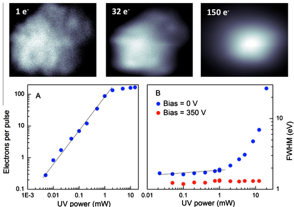
Fig. 2. (A) Beam current as a function of UV power. (B) Dependence of the FWHM of the ZL peak on the UV power for two different Wehnelt bias voltages. In the top panels of the figure, the images of the tip taken for three different illuminating UV powers are shown.
